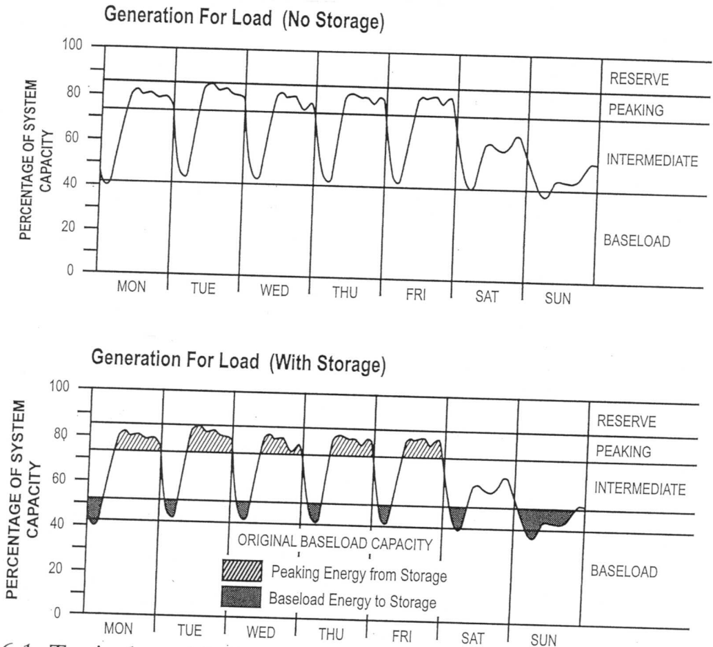
Figure 16.1. Typical weekly load curve of an electric utility. Source: National Academy of Sciences (1976).
