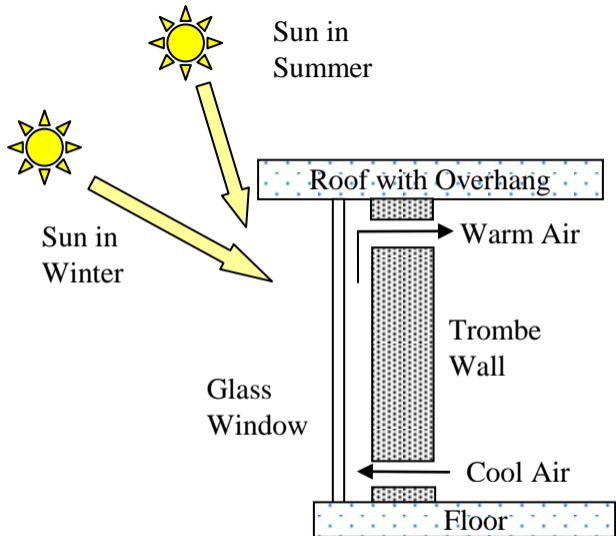
Figure 6.5 Representation of a Trombe wall.
