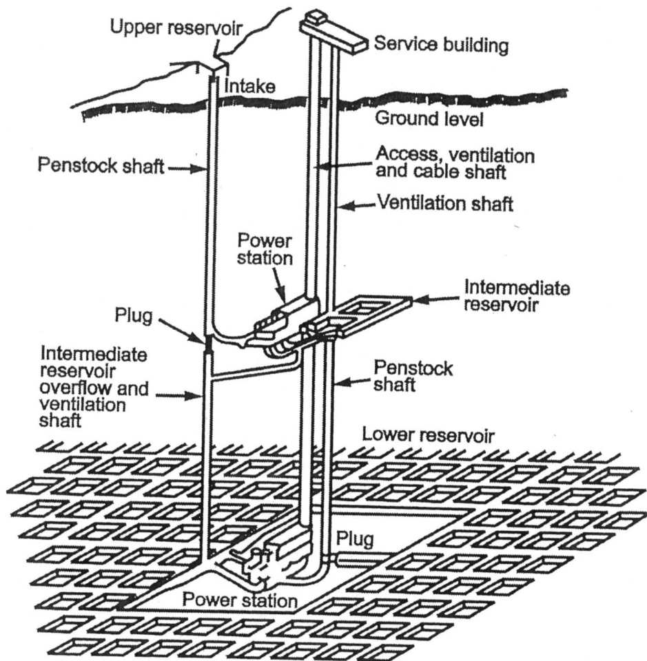
Figure 16.6a. Schematic illustrations of several energy storage technologies: Aboveground and underground pumped hydro . Source: Jensen and Sorensen (1984). Reprinted with permission of Elsevier.
