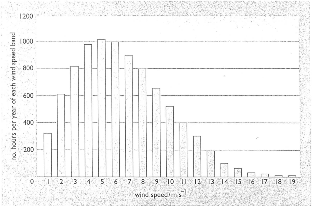
Figure 7.30 A typical wind speed frequency distribution
