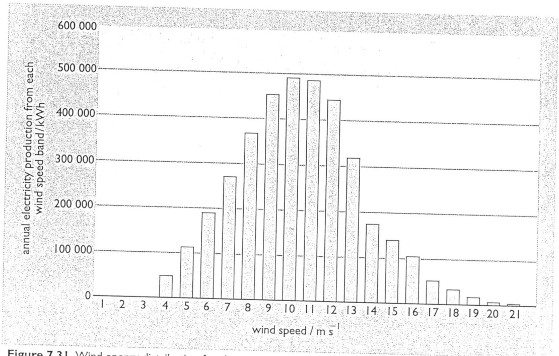
Figure 7.31 Wind energy distribution for the same site as in Figure 7.30, showing energy produced at this site by a wind turbine with the wind speed-power curve shown in Figure 7.29
