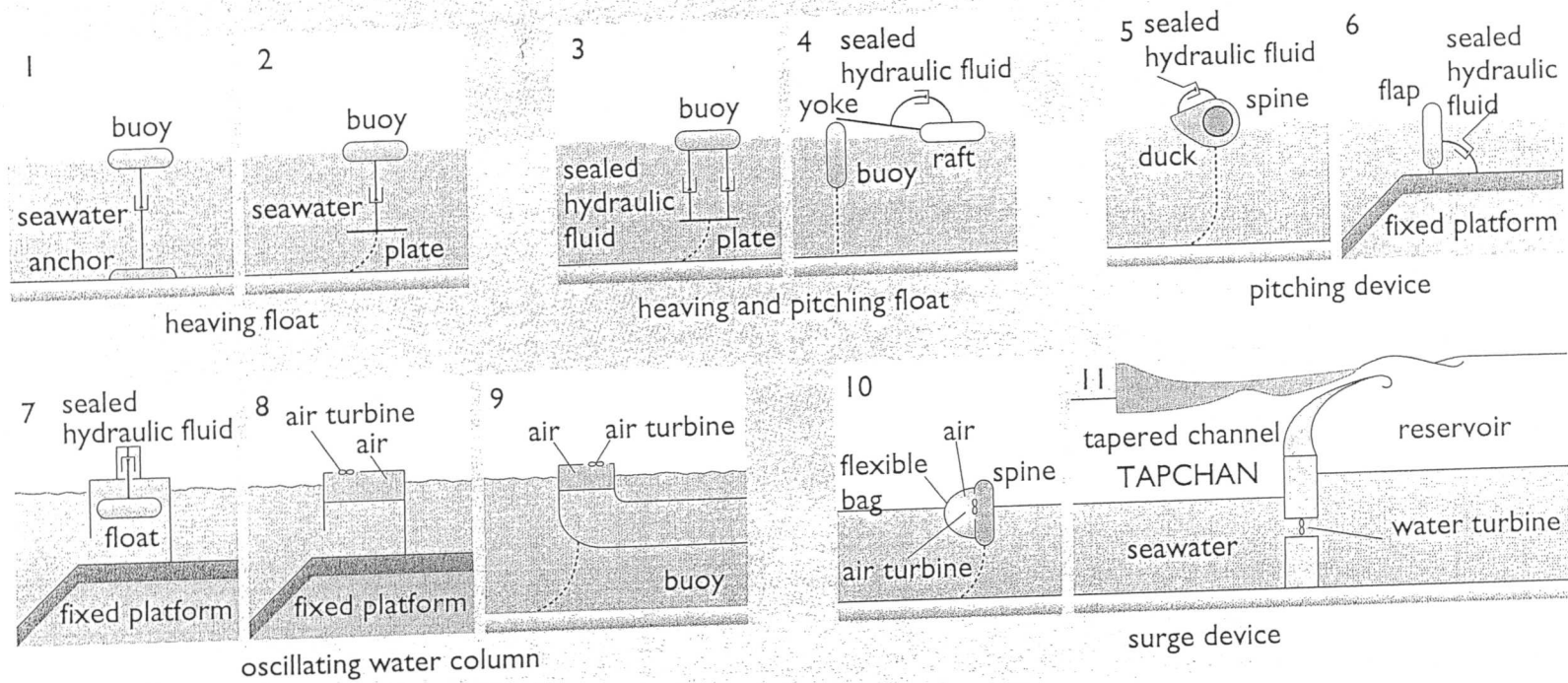
Figure 8.14 Schematic representations of various types of wave energy converter (Source: based on Falnes and Løvseth, 1991)
