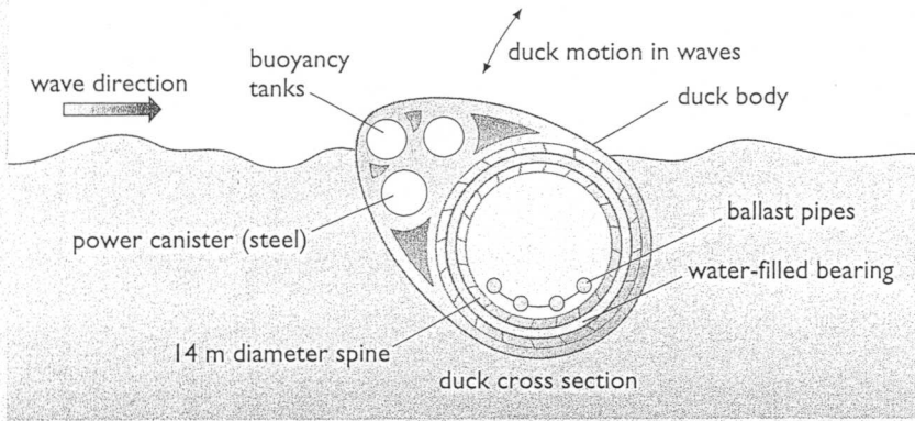
Figure 8.23 (a) The Edinburgh Duck wave energy converter (b) Duck model being tested in a wave tank (c) A scale model of the Duck being tested in Loch Ness, Scotland
