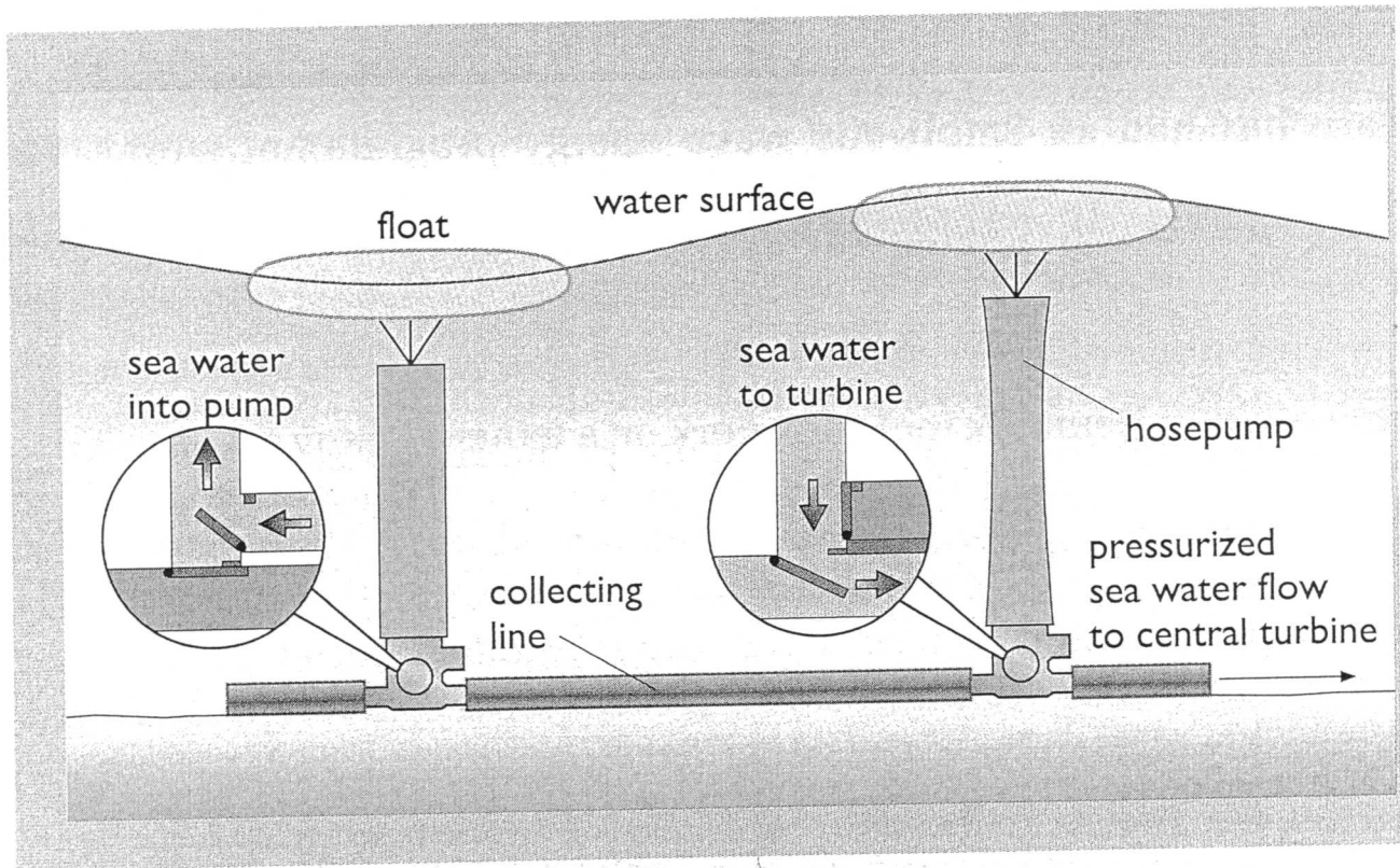
Figure 8.30 Swedish hose pump wave energy converter
