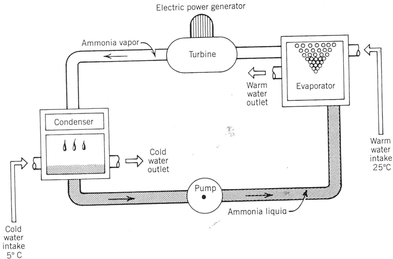
Figure 7.10 An OTEC heat engine using ammonia as a working fluid. The turbine is driven by the ammonia vapor and is connected to a generator to produce electricity. The warm water is drawn from the ocean surface; the cold water from a depth of 1000 m. (Figure supplied by the Solar Energy Research Institute.)
