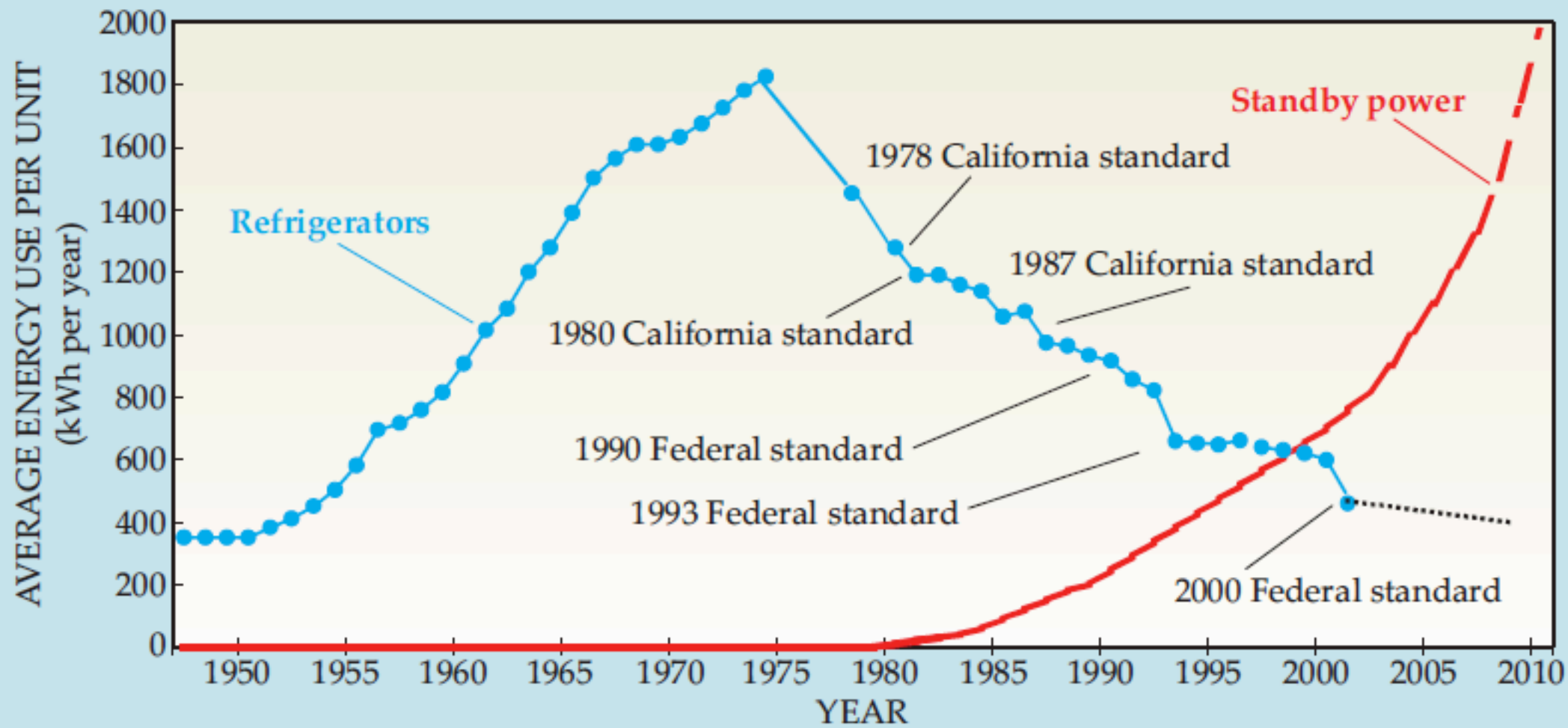
Figure 3. Energy use for refrigerators and standby electronics. Regulation and financial incentives have decreased the energy consumption of household refrigerators. But the decrease has been offset by the growing energy consumption by electronics in standby mode. (Data courtesy of Arthur Rosenfeld, California Energy Commission.)
